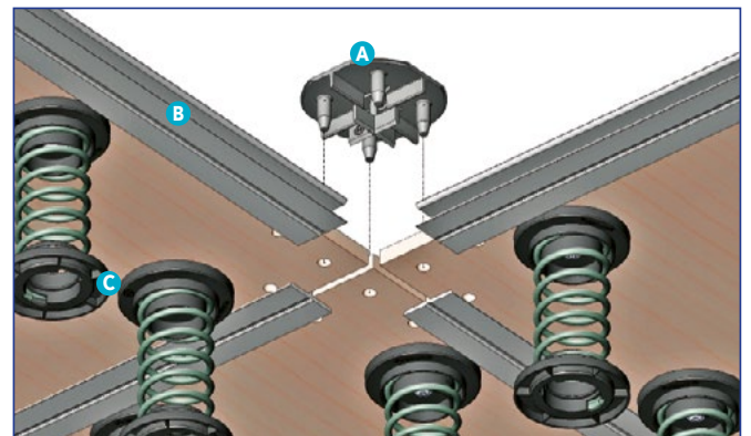
A/ Locking plate - B/ Fastening section - C/ Springs
