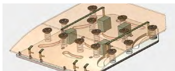
13 high-elasticity springs designed specially for vaulting
